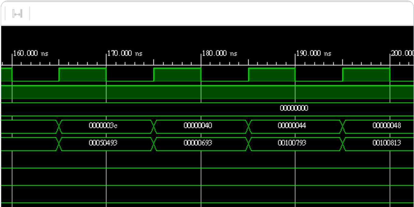
Load-use stall clk, rst_n, errors, pc, if_instr, load_use_stall, if_id_stall, id_ex_flush
