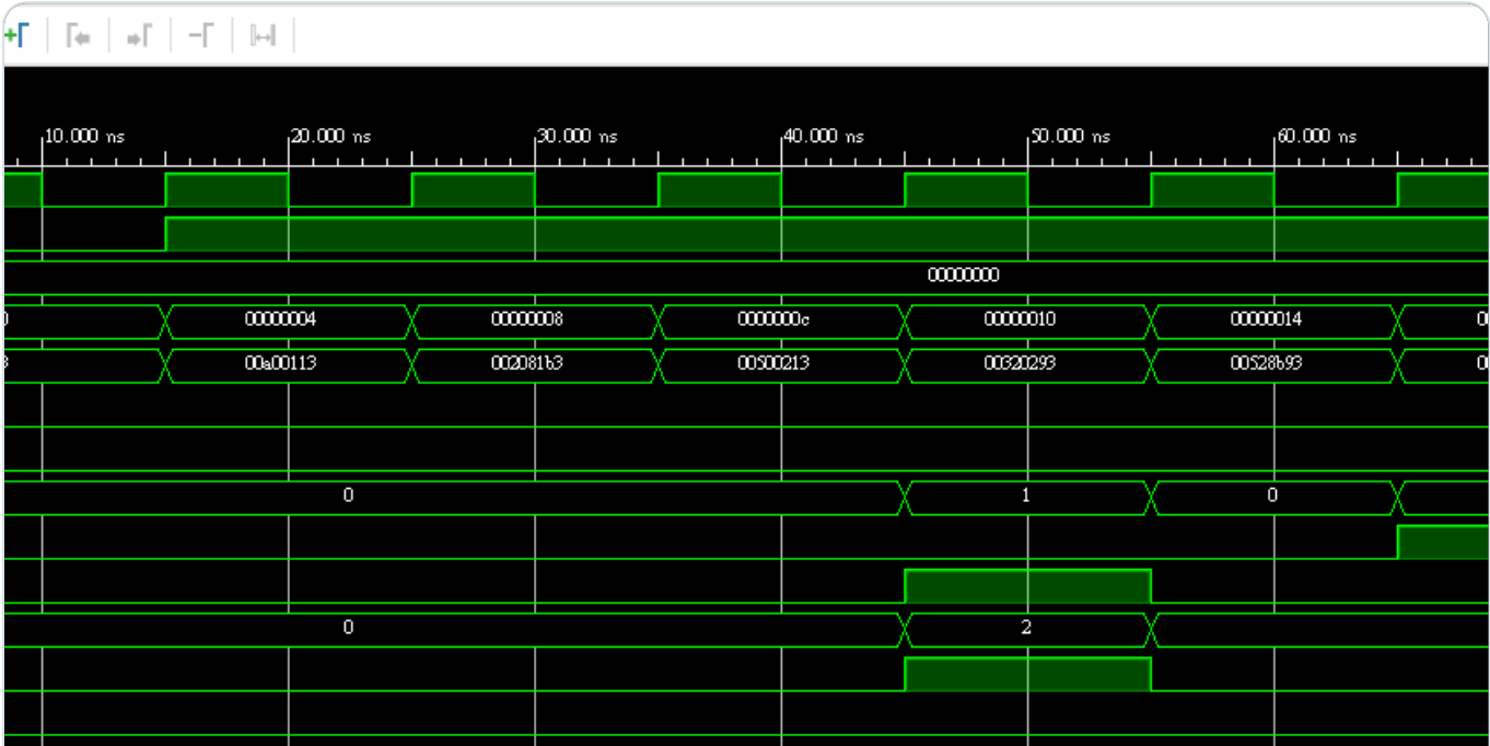
基本五級管線模擬波形 clk, rst_n, errors, pc, if_instr, load_use_stall, flush, forward_a, forward_b
